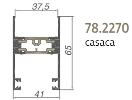
78.1600 marco 4 carriles
